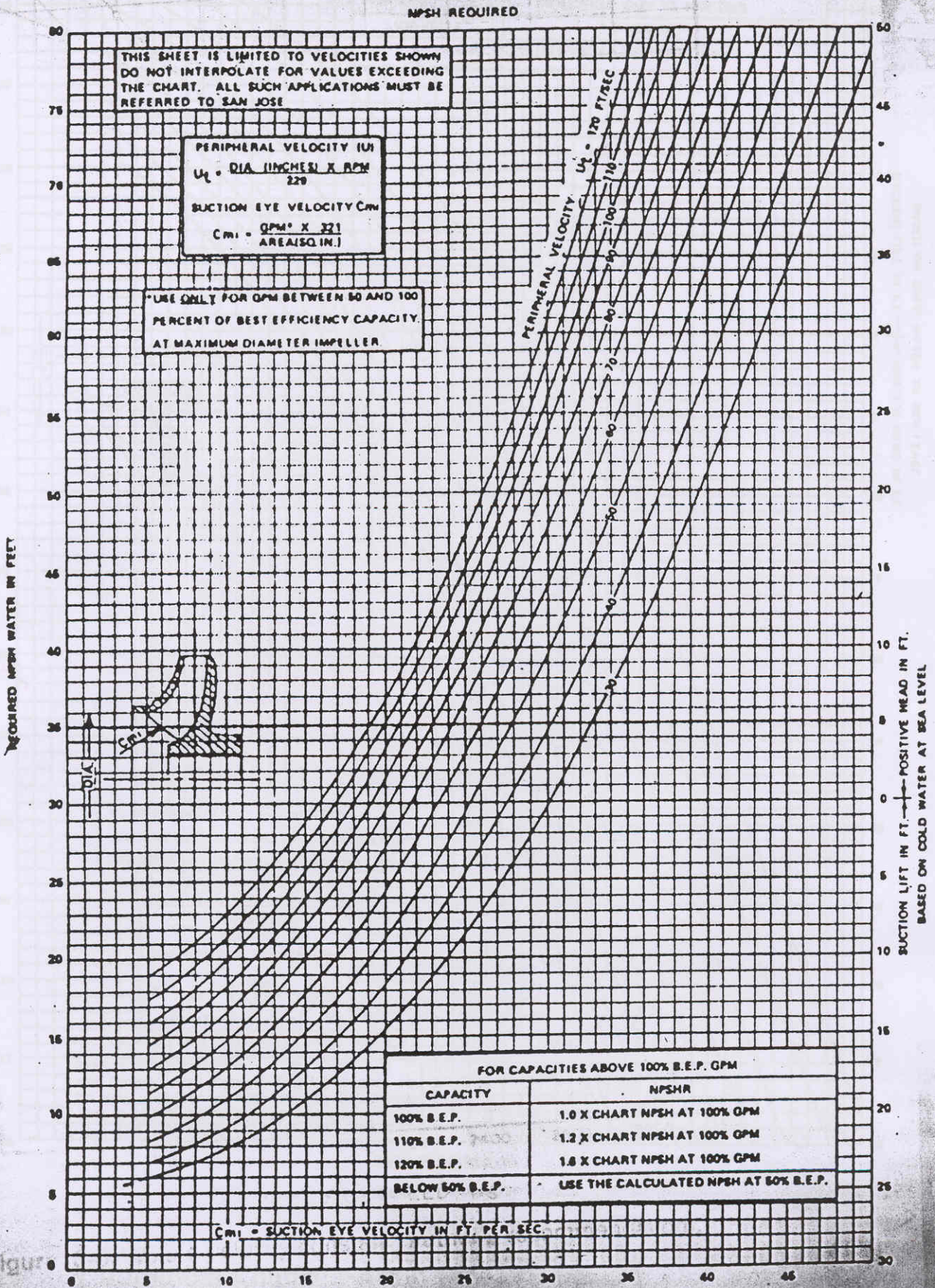
Figure 3-6. NPSHR prediction chart.
